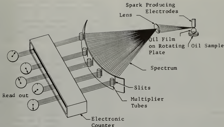
FIGURE 10-75. Spectrometric Analysis of Metals
